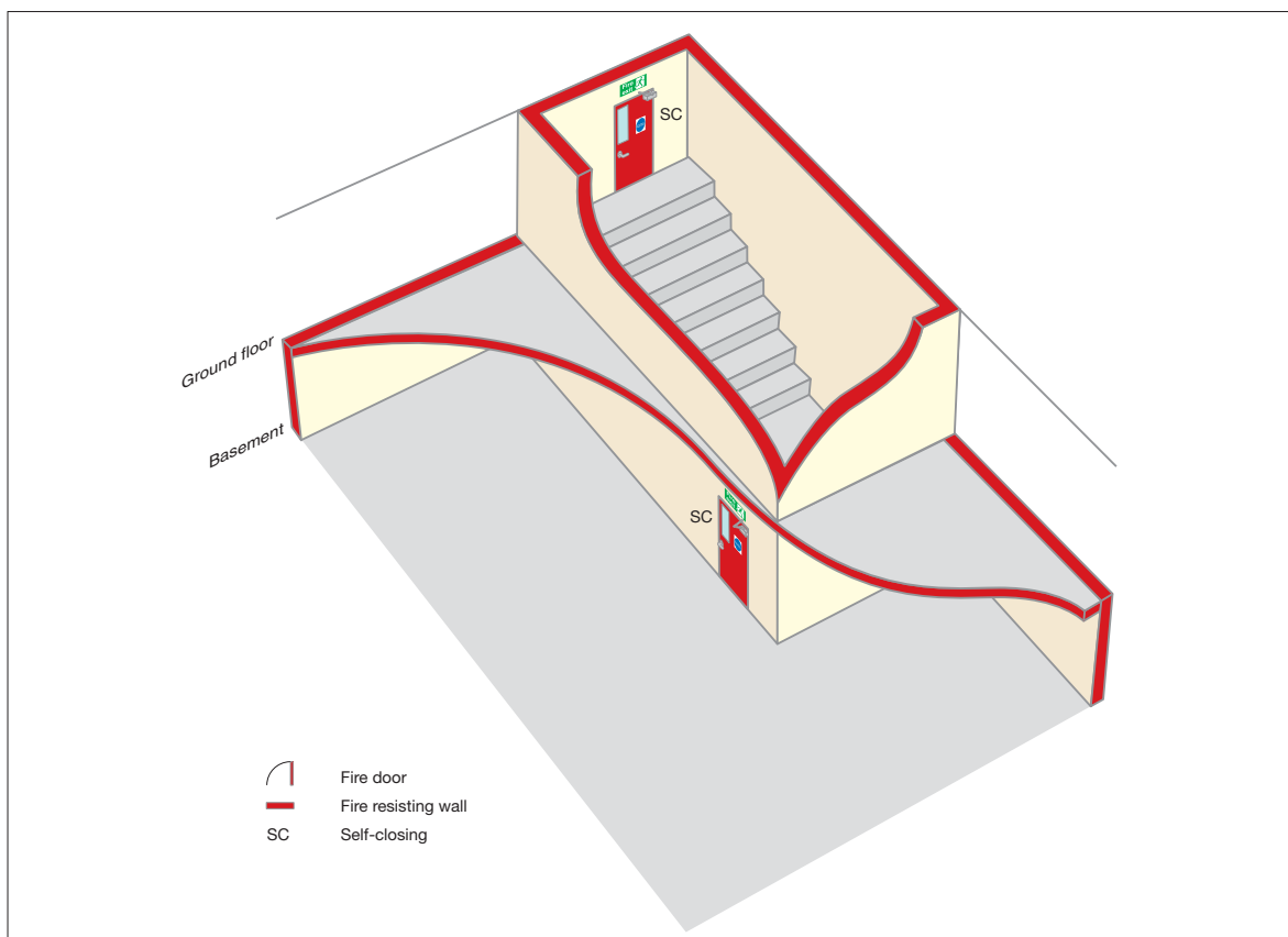
Figure 32: Basement protection
